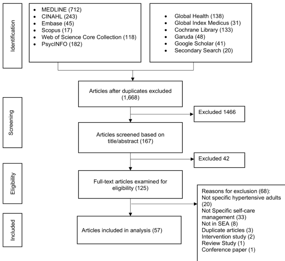
Figure 6 PRISMA flowchart.
